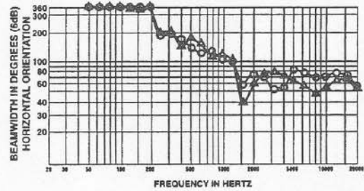
FIGURE 6 — Sx200a Directivity Response (anechoic environment)
